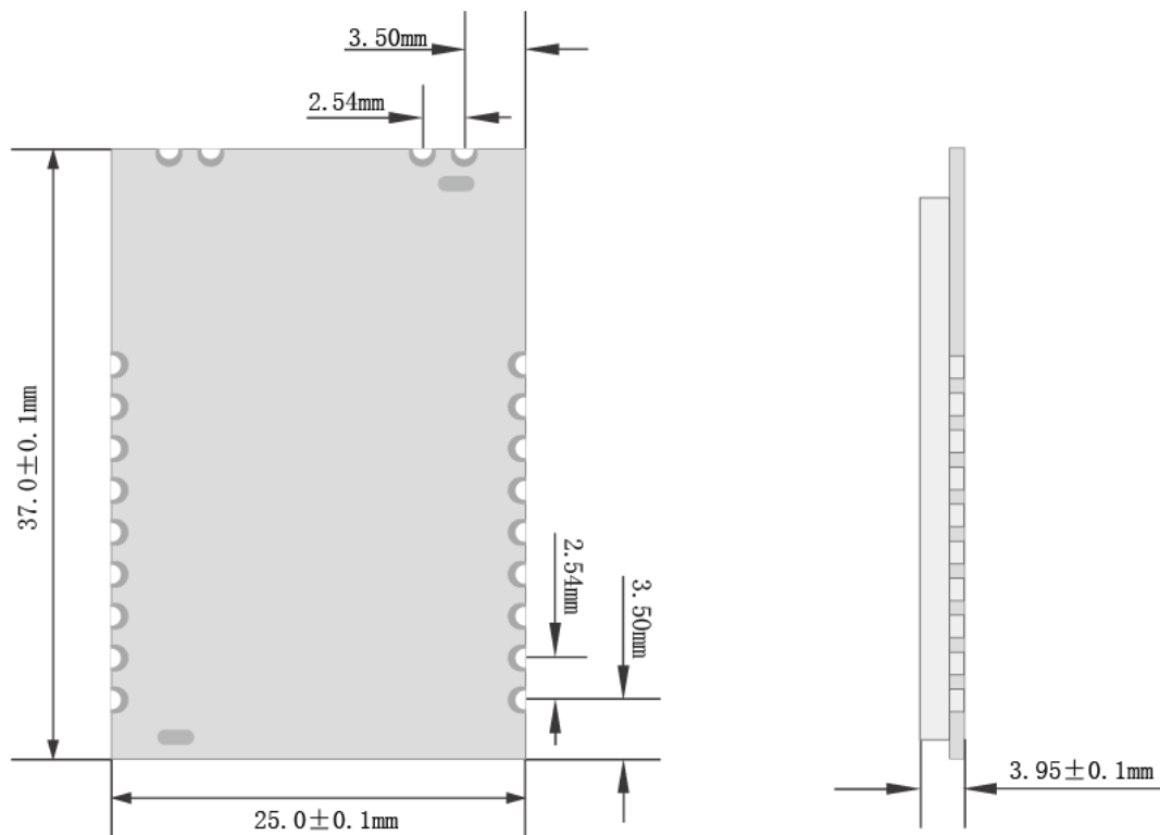
Figure 2: Module size
