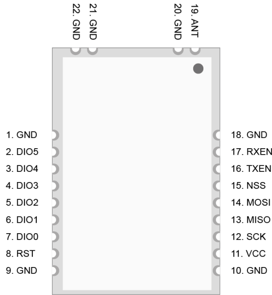
Figure 1: Pins Diagram
